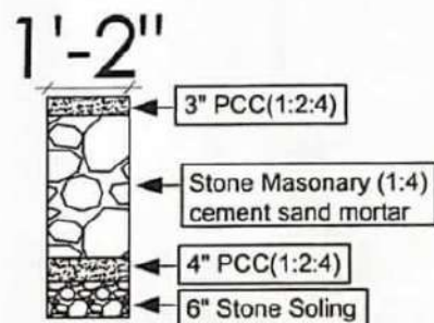
Cross Section of Wall 4, 5, 6 & 7 (different in height and lenght according to estimate)
