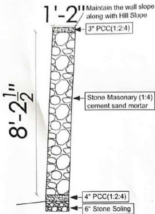
Cross Section of Wall 1
