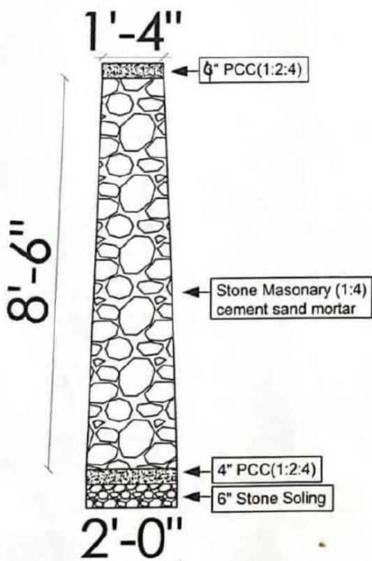
Cross Section of Wall 3
